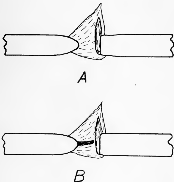
FIG. 1. Sketches showing the appearance of the direct-current arc with coaxially aligned electrodes: (A) With no negative "tongue"; (B) with negative "tongue."
